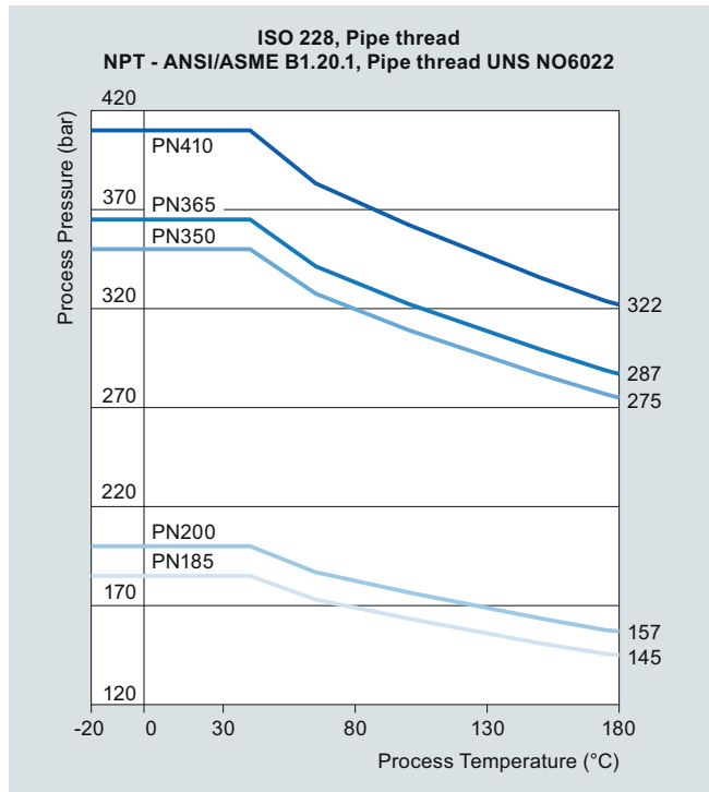
ISO 218 and NPT flanges stainless steel (PN 185 ... PN 410)
