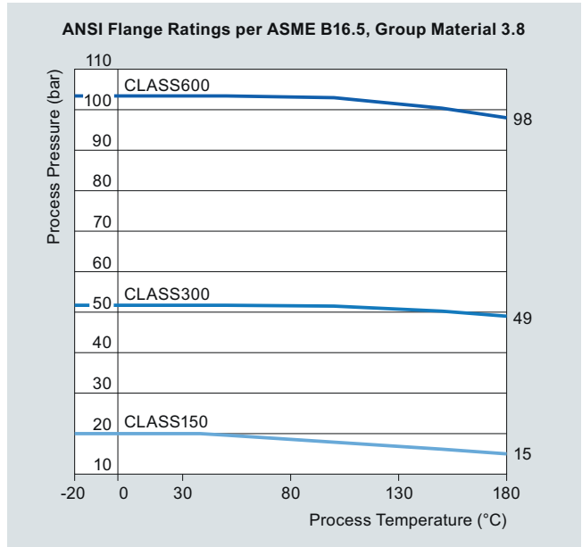
ASME flanges B16.5 Hastelloy C22
