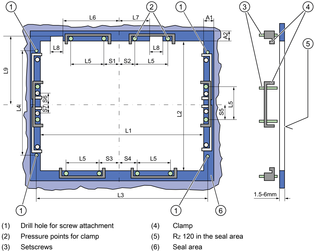
Figure 1-2 Drill holes for the screws and pressure points for the clamp screws
